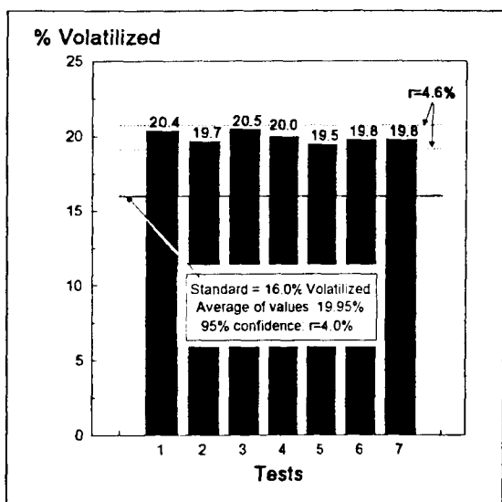
Figure 5 - First study of repeatability.
