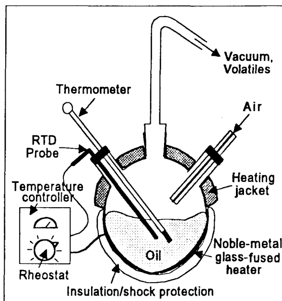
Figure 3 - Noble-metal glass-fused heater modified-Noack volatility cell.
