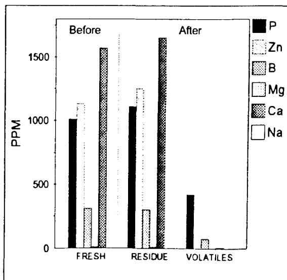
Figure 16 - Results of ICP analyses of the three samples of the SAE 30 before and after volatilization.
