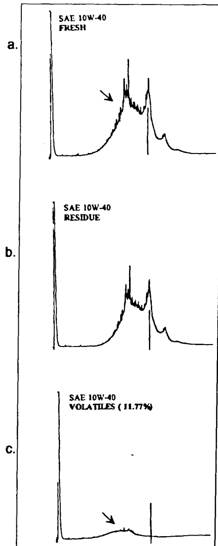
Figure 12 - Gas chromatograms of a modified-Noack test of the SAE 10W-40 synthetic or parasythetic engine
