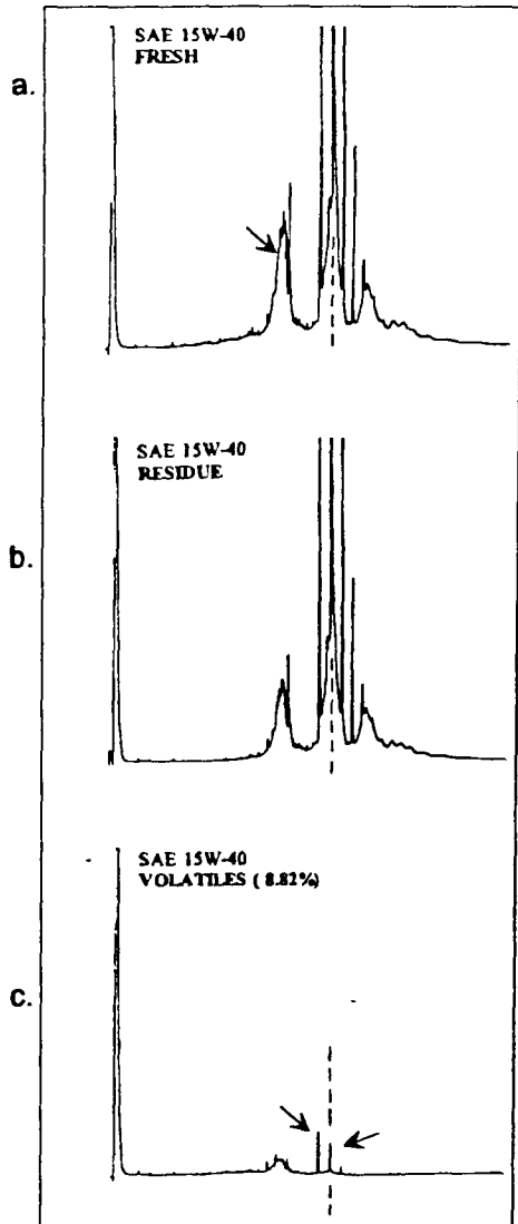
Figure 11 - Gas chromatograms of a modified-Noack test of the SAE 15W-40 synthetic engine oil..
