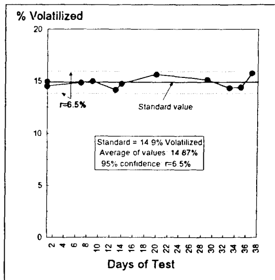
Figure 6 - Second study of repeatability from laboratory quality assurance data.
