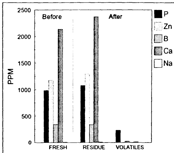
Figure 17 - Results of ICP analyses of the three samples of the SAE 15W-40 before and after volatilization.
