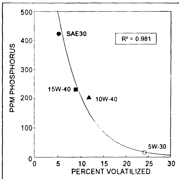
Figure 20 - Crossplot of phosphorous concentration in volatile samples and the percent volatilized.
