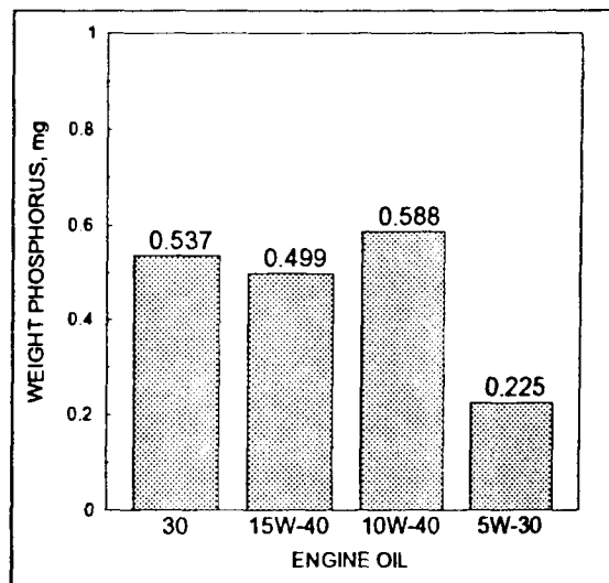
Figure 21 - Comparison of total phosphorous weight in volatile samples from modified-Noack tests.
