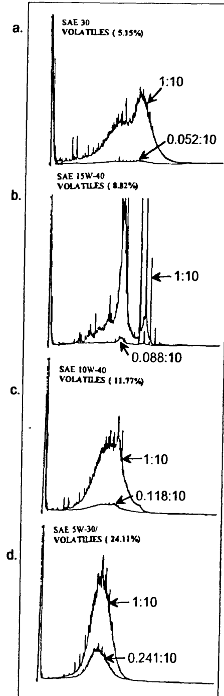
Figure 14 - GCs of the volatile components of the four commercial engine oils at two levels of concentration.
