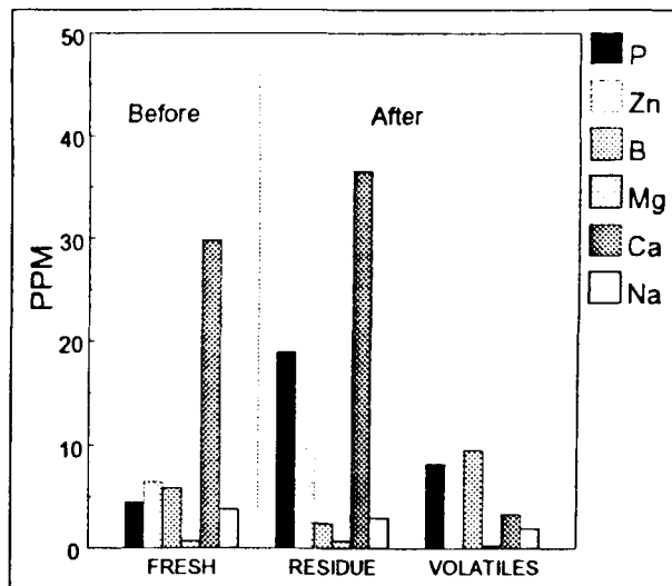
Figure 15 - Results of ICP analyses of the three samples of the Noack reference oil before and after volatilization.
