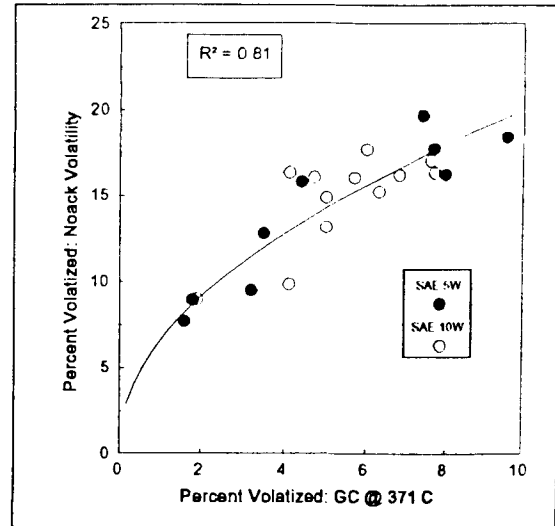
Figure 2 - Noack correlation with GC at 371°C.
