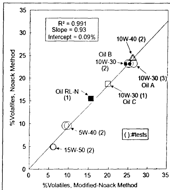
Figure 7 - Correlation of Noack and modified-Noack results.
