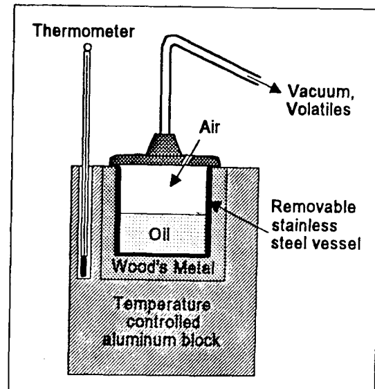
Figure 1 - Noack's volatilizing chamber.
