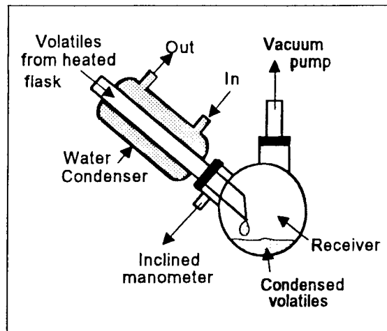
Figure 4 - Volatiles condensation and collection.
