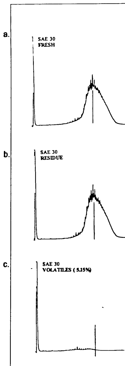
Figure 10 - Gas chromatograms of the three components of a modified-Noack test of the SAE 30 engine oil.
