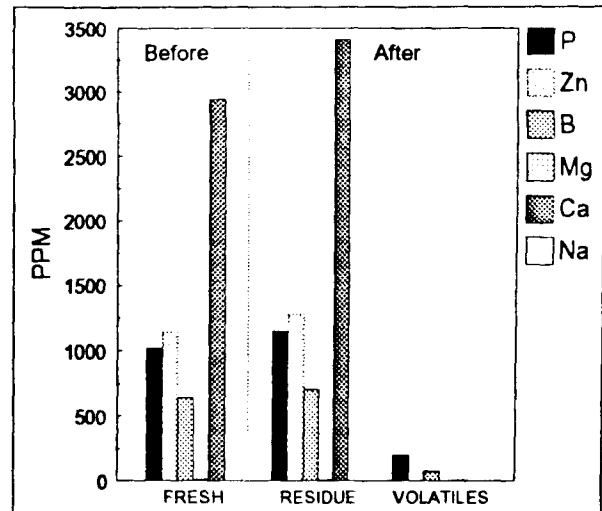
Figure 18 - Results of ICP analyses of the three samples of the SAE 10W-40 before and after volatilization.
