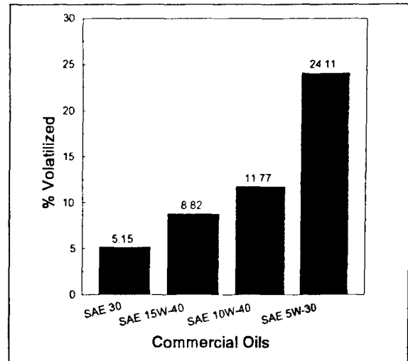
Figure 8 - Percent volatilized of four chosen commercial engine oils.
