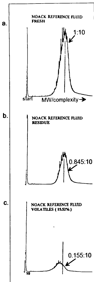
Figure 9 - Gas chromatograms of the three components of a modified-Noack test of the Noack reference oils at dilutions proportional to their fraction of the fresh oil.
