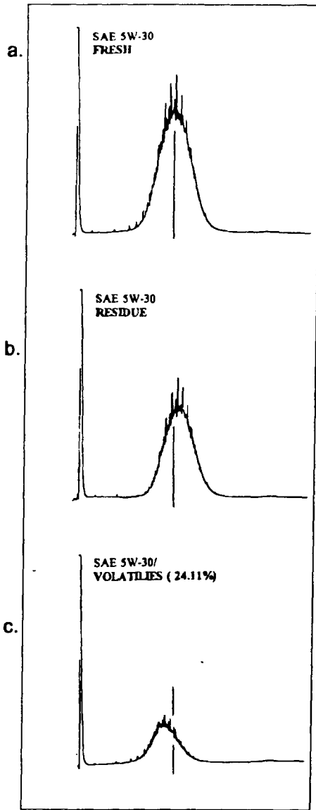
Figure 13 - Gas chromatograms of a modified-Noack test of the SAE 5W-30 mineral-based engine oil.
