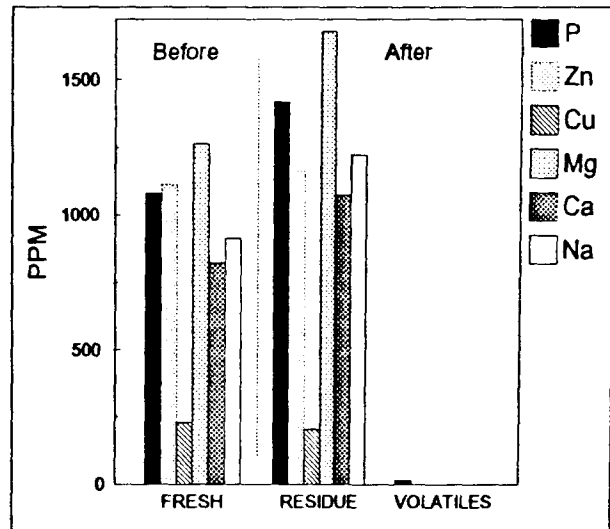
Figure 19 - Results of ICP analyses of the three samples of the SAE 5W-30 before and after volatilization.
